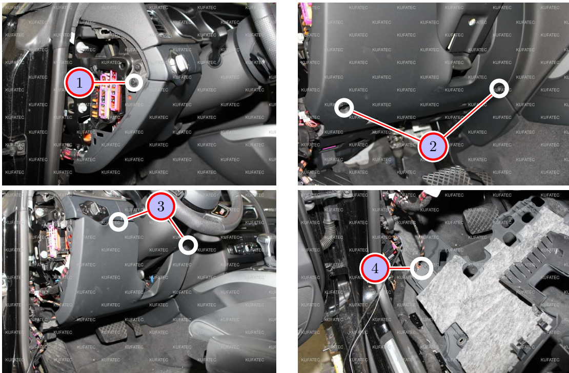
Figure 5: Removing trim panel driver's side
